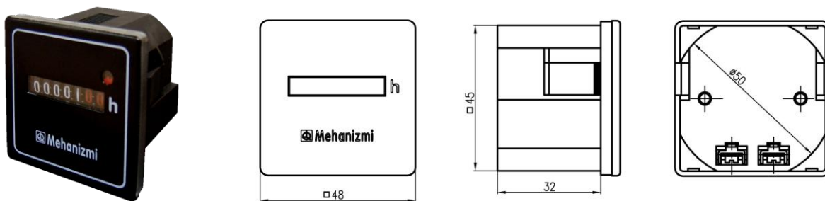
HK 46 – mounting F
