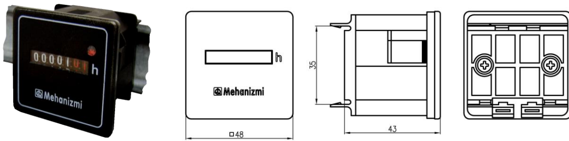
HK 46 – mounting D
