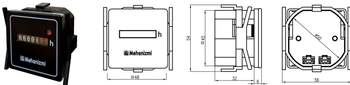
HK 46 – mounting G
