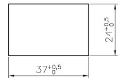
Panel cut-out
