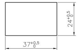
Panel cut-out
