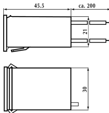
Mounting with fork clamp and cutout.
