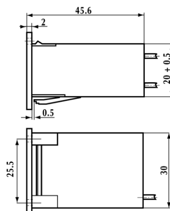
Mounting with fork clamp and cutout.
